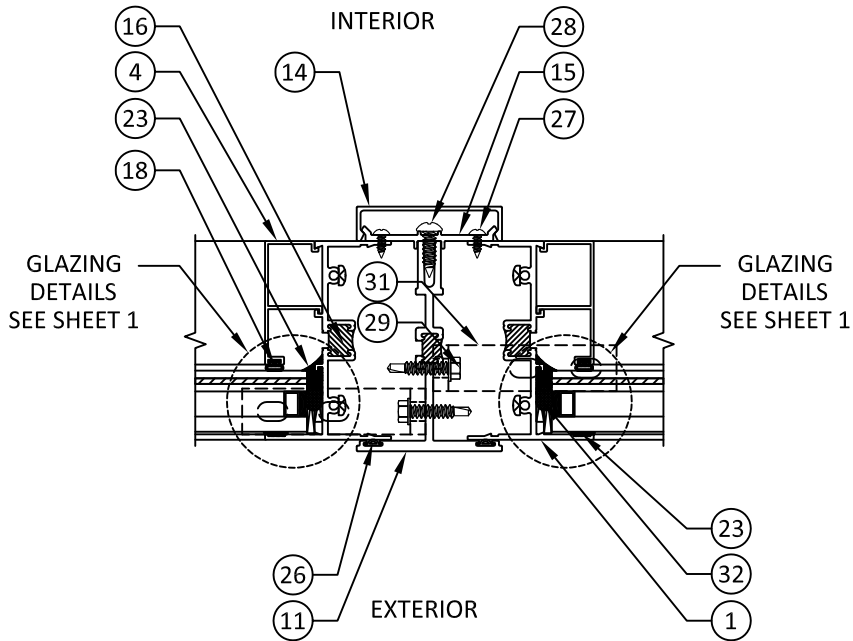
B 6 HORIZONTAL SECTION MULLION ( SPAN UP TO 72" )
