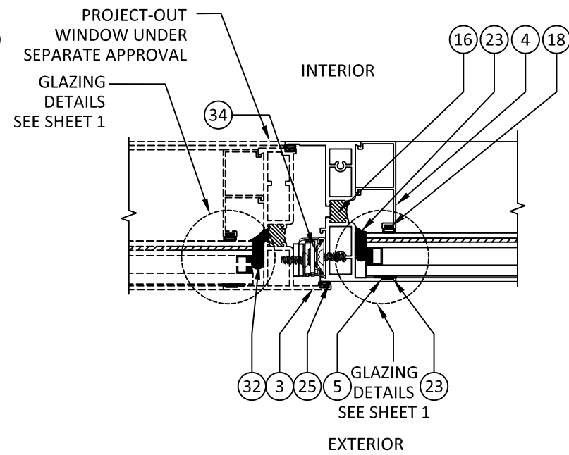
F 6 HORIZONTAL SECTION MEETING RAIL PO-FX ( MAX SPAN 60" )
