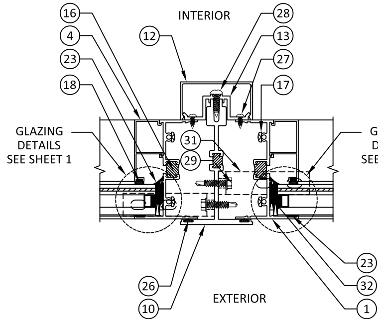
A 6 HORIZONTAL SECTION MULLION ( SPAN ABOVE 72" )
