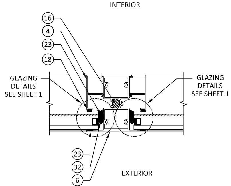
C 6 HORIZONTAL SECTION MEETING RAIL FX-FX ( MAX SPAN 72" )
