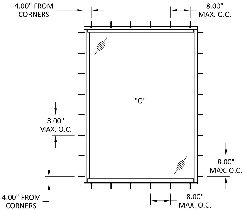
ANCHOR LAYOUT FIXED WINDOW THROUGH FRAME INSTALLATION
