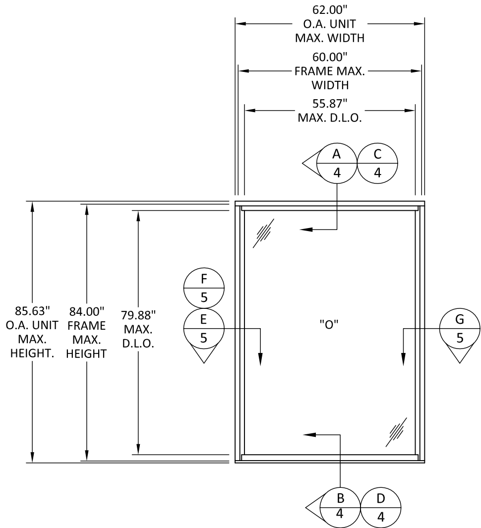
EXTERIOR ELEVATION FIXED WINDOW
