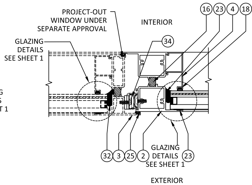
E 6 HORIZONTAL SECTION MEETING RAIL PO-FX ( MAX SPAN 72" )
