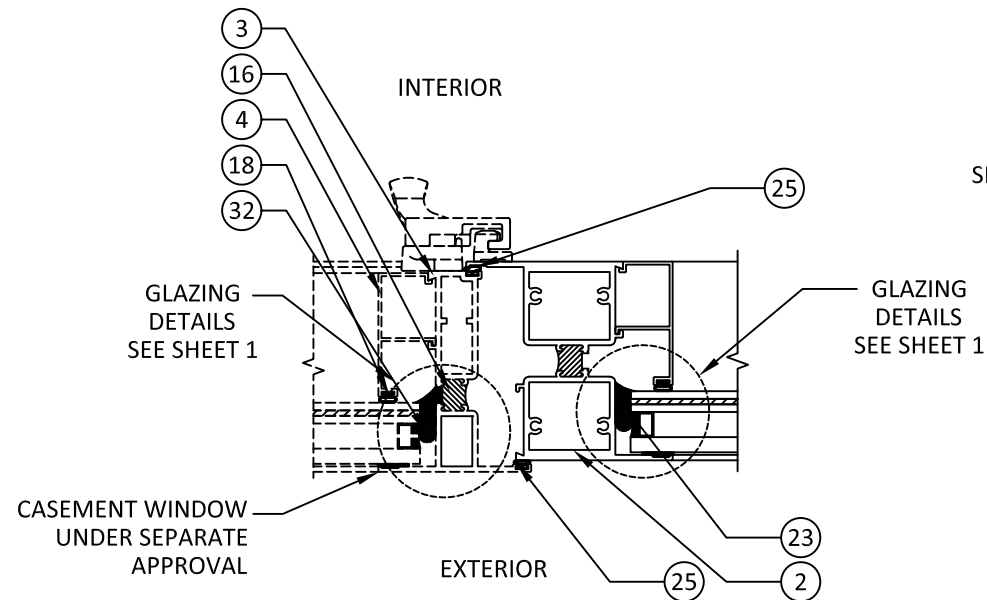
D 6 HORIZONTAL SECTION MEETING RAIL AT CS-FX ( MAX SPAN 72" )
